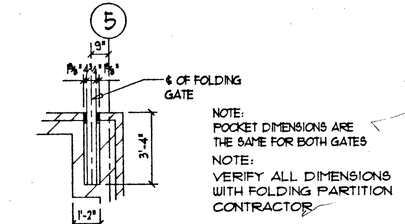
B POCKET DETAIL A-3 SCALE 1/2" = 1'-0"
