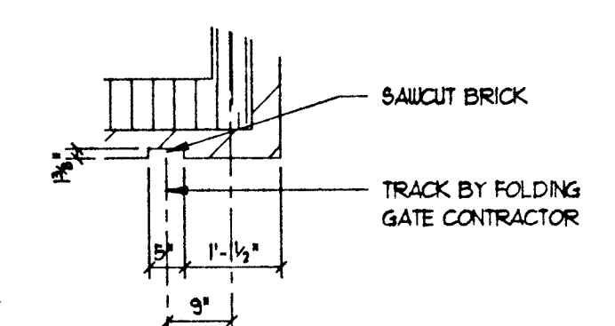
C POCKET DETAIL A-3 SCALE 1/2" = 1'-0"
