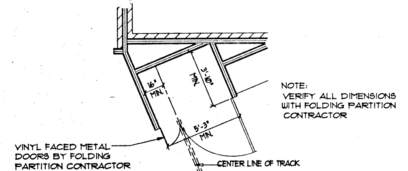
A POCKET DETAIL A-3 SCALE 1/2" = 1'-0"
